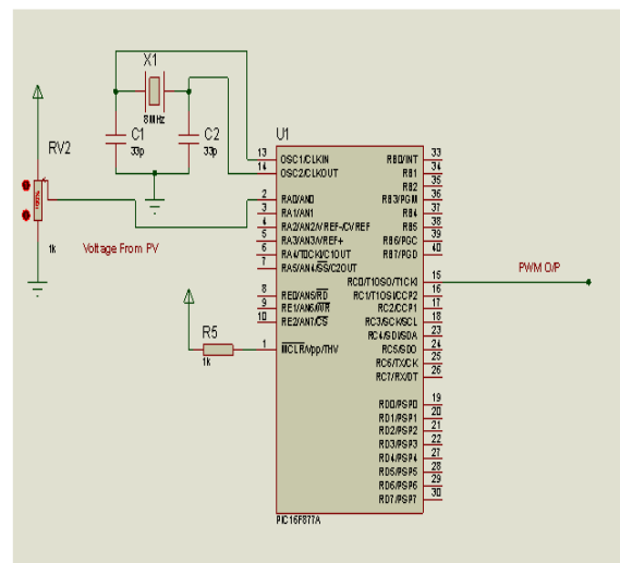
Fig. 14. Hardware Implementation-2
