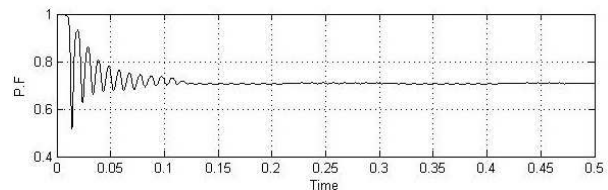
Fig. 9. Output power factor .
