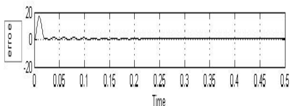
Fig. 22 Grid connected load Error Curve
