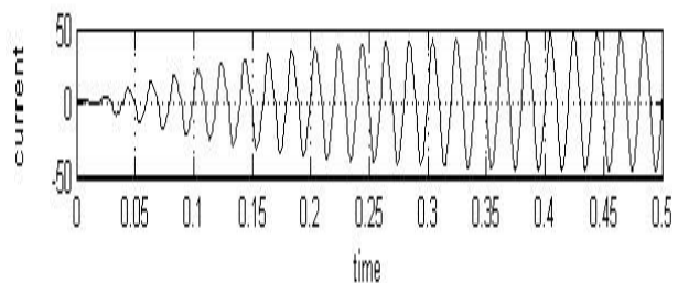
Fig. 20 Grid connected load current Curve
