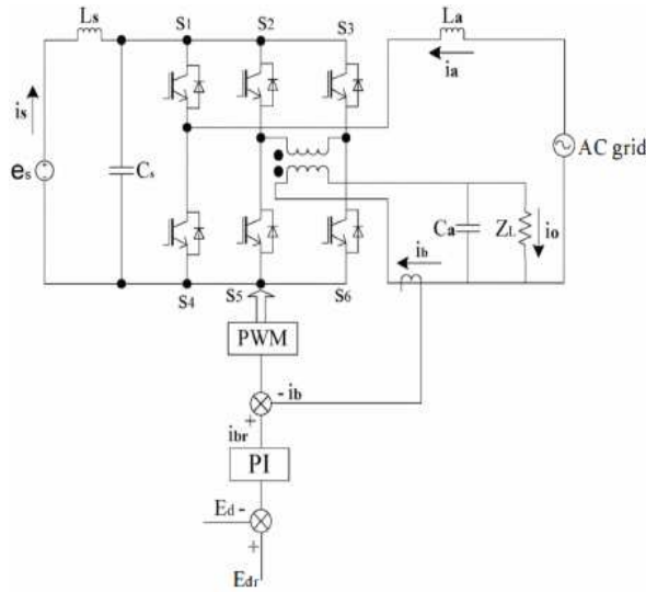
Fig. 4 Improved type PWM Inverter Control System.
