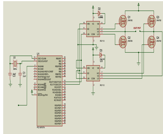
Fig. 13. Hardware Implementation-1
