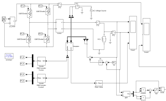
Fig. 17 Single-phase PV grid-connected generation system
