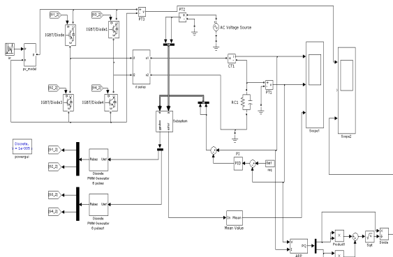
Fig.5 Single-phase PV grid-connected generation system
