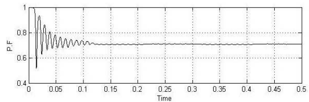
Fig. 19. Output power factor
