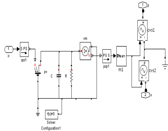
Fig. 6 PV Model
